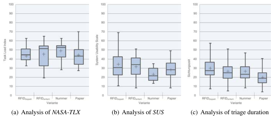
Figure 3: Evaluation results
